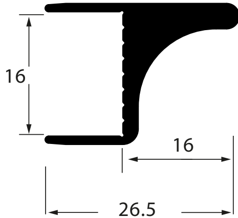
PRO-GO452A
