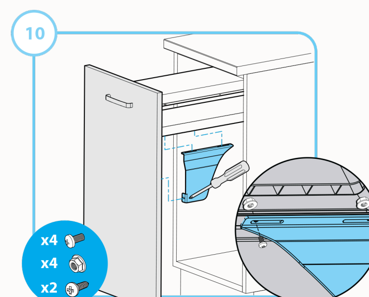
Attach door brackets
