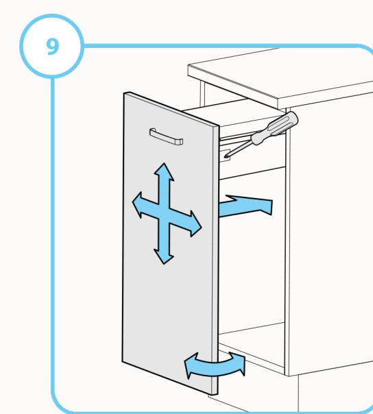
Re-install drawer assembly and adjust door
