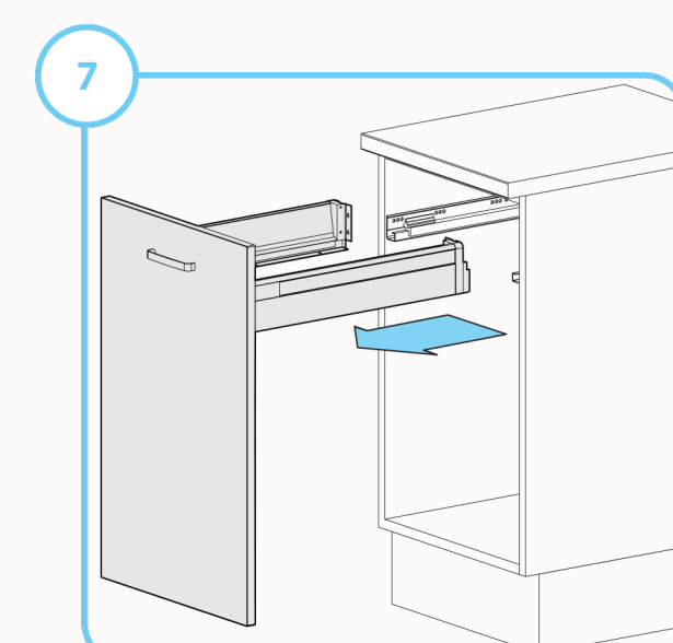
Remove drawer assembly
