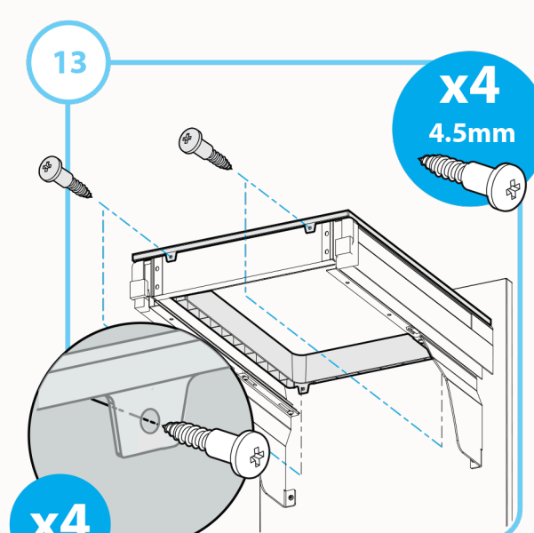
Attach tray with stepped screws
